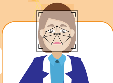
Biometrics verification
